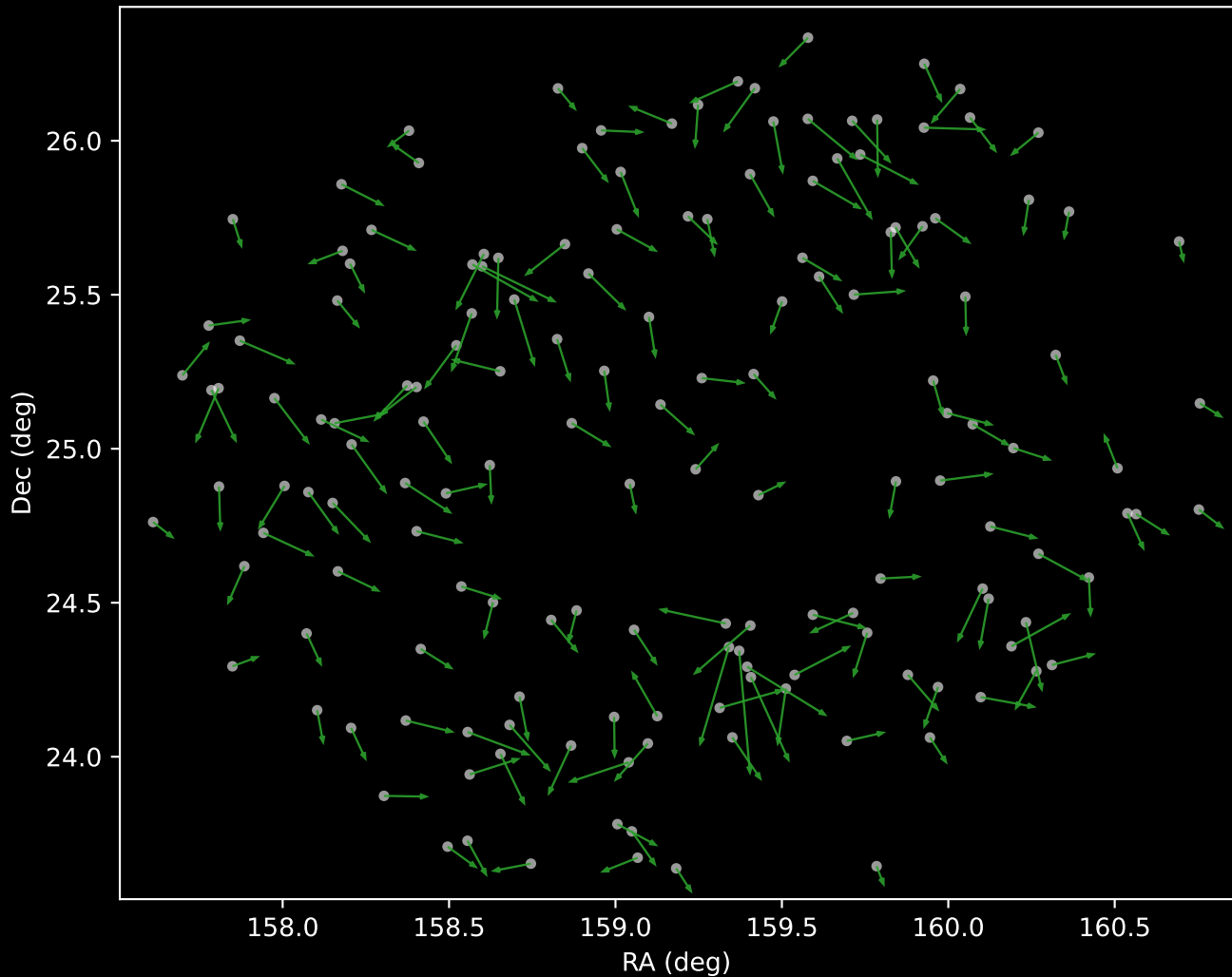
APOGEE DR17 Cluster 4 Proper Motion Vectors (n=159)
