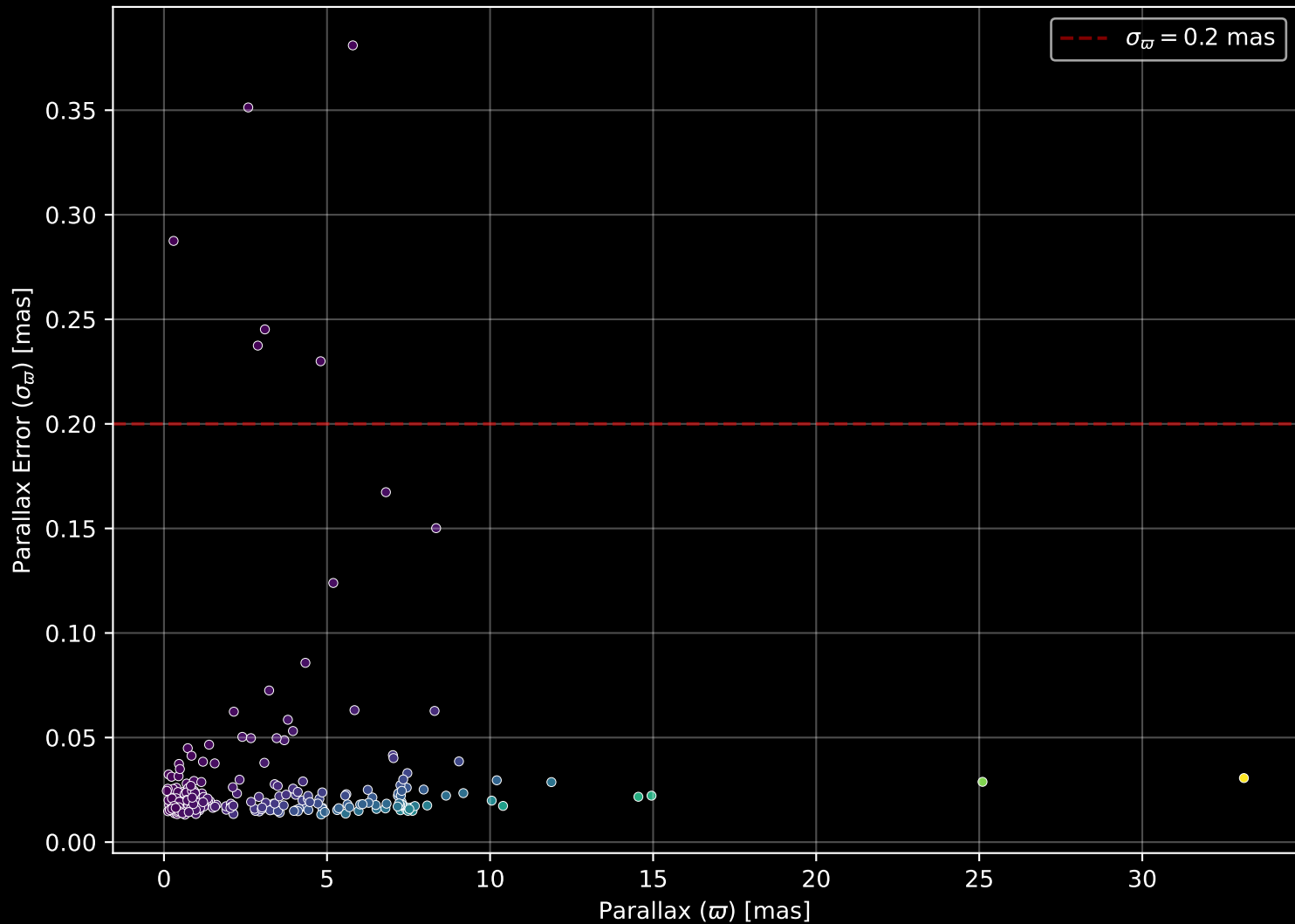
APOGEE DR17 Field: [K2_C4_168-21] Parallax Quality (n= 295)
