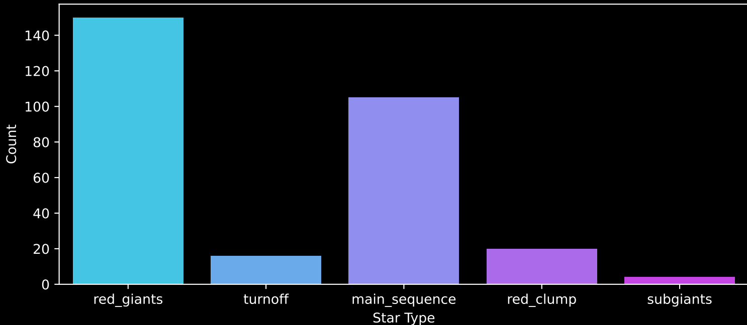
APOGEE DR17 Field: [K2_C4_168-21] Count plot of Star Type
