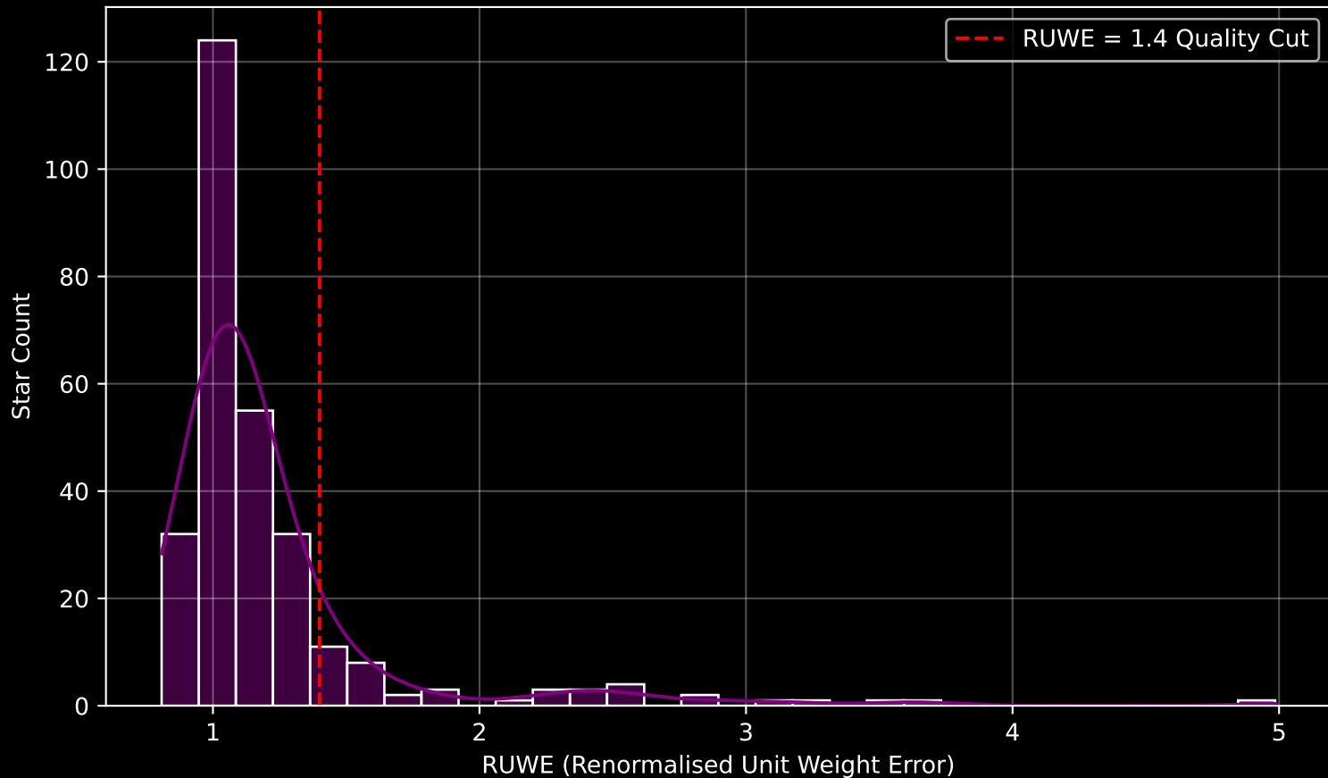
GAPOGEE DR17 Field [K2_C4_168-21] RUWE Distribution (n= 285)
