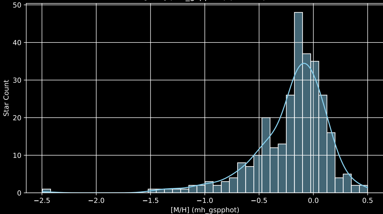
APOGEE DR17 Field: [K2_C4_168-21 [M/H] (mh_gspphot) (n= 293)
