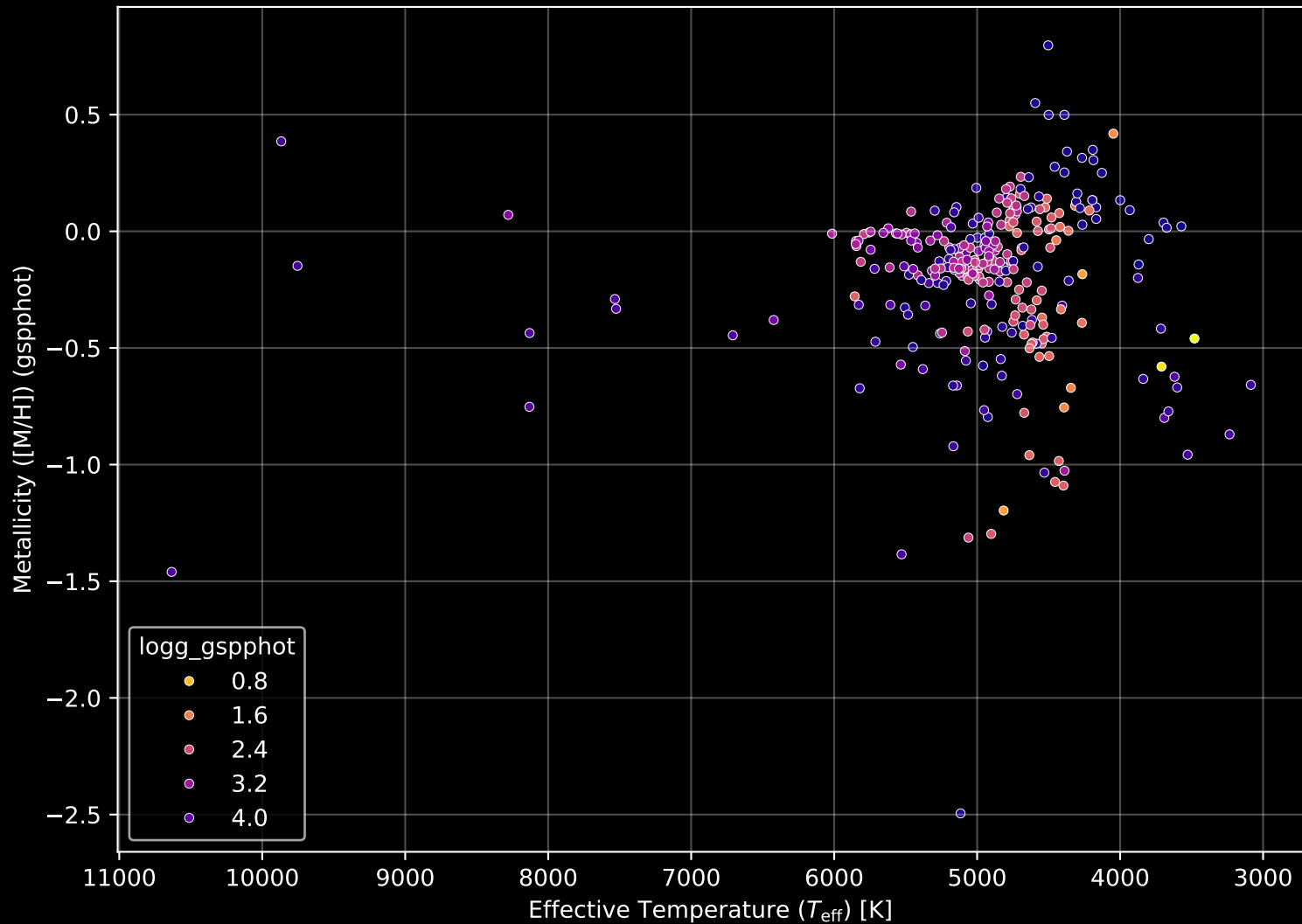
APOGEE DR17 Field: [K2_C4_168-21] Stellar Population Parameters (n= 295)
