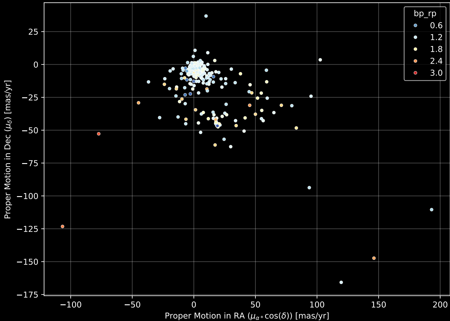
APOGEE DR17 Field: [K2_C4_168-21] Proper Motion Diagram (n= 295)
